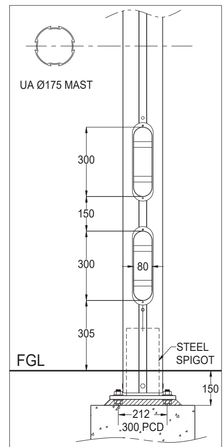
BASE DETAIL
